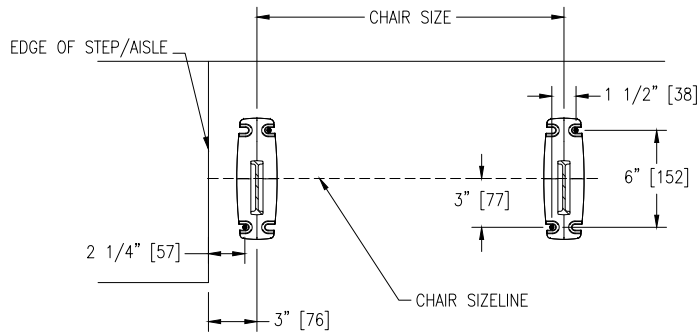
ANCHOR BOLT LOCATIONS
