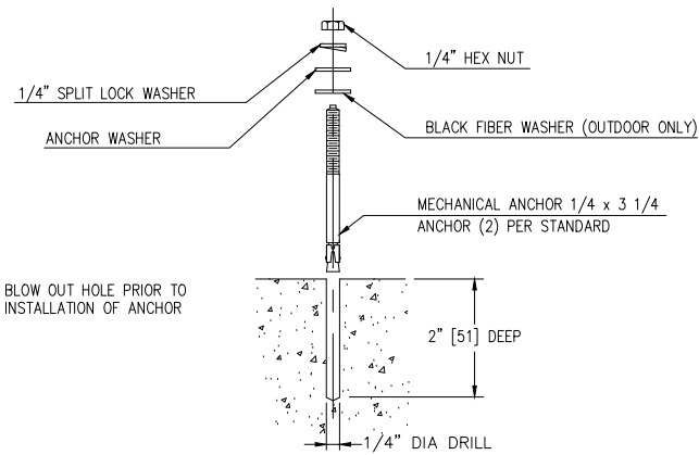
FLOOR MOUNT ANCHOR DETAIL
